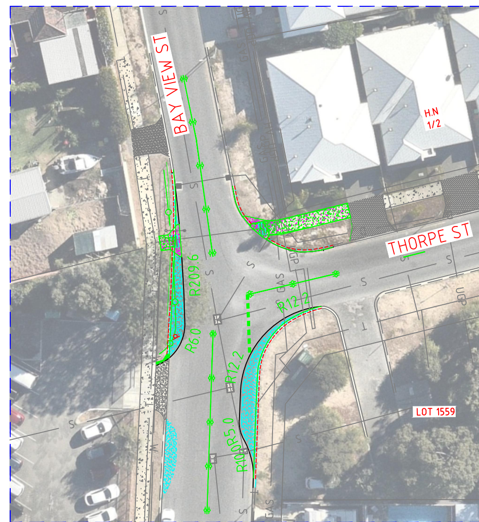
PROPOSED VERGE WIDENING
