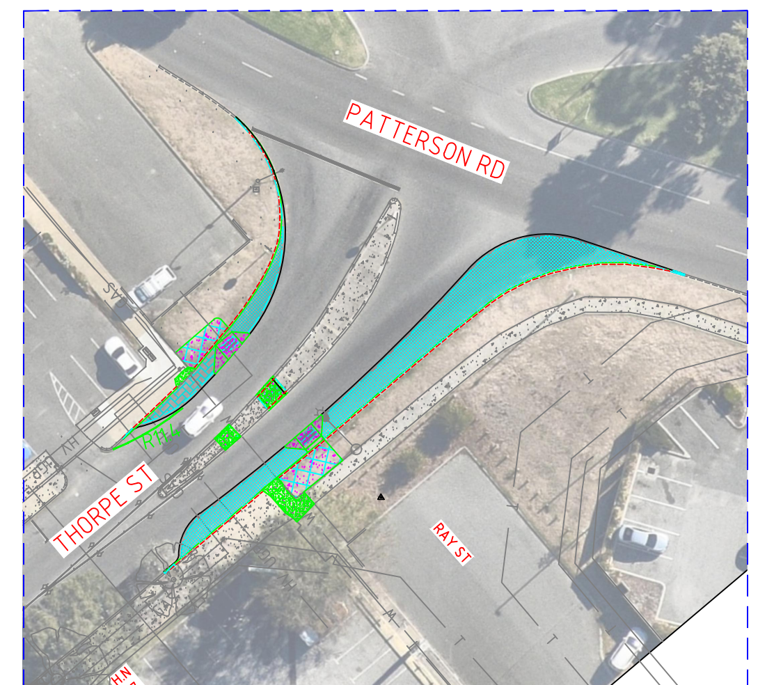
PROPOSED VERGE WIDENING
