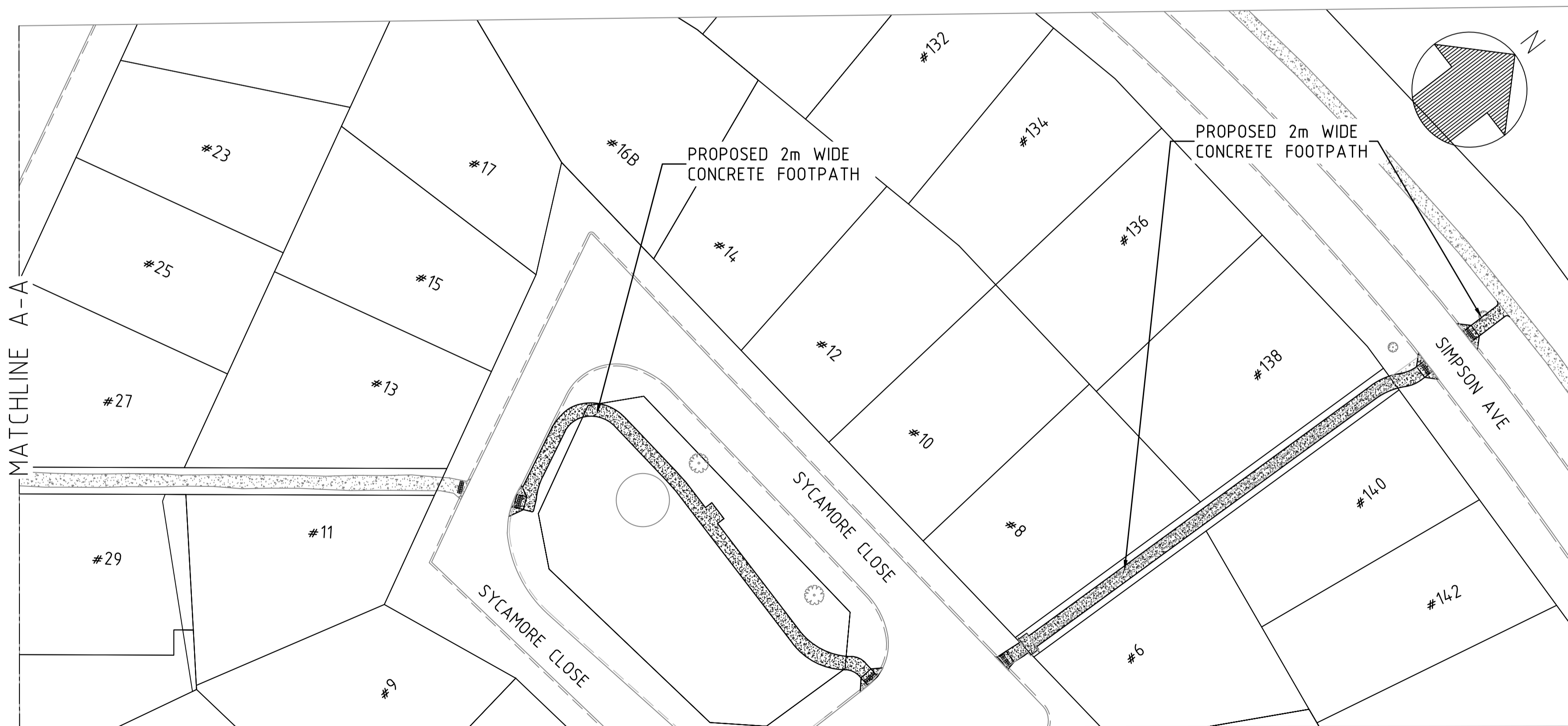
PLAN SCALE 1:500
