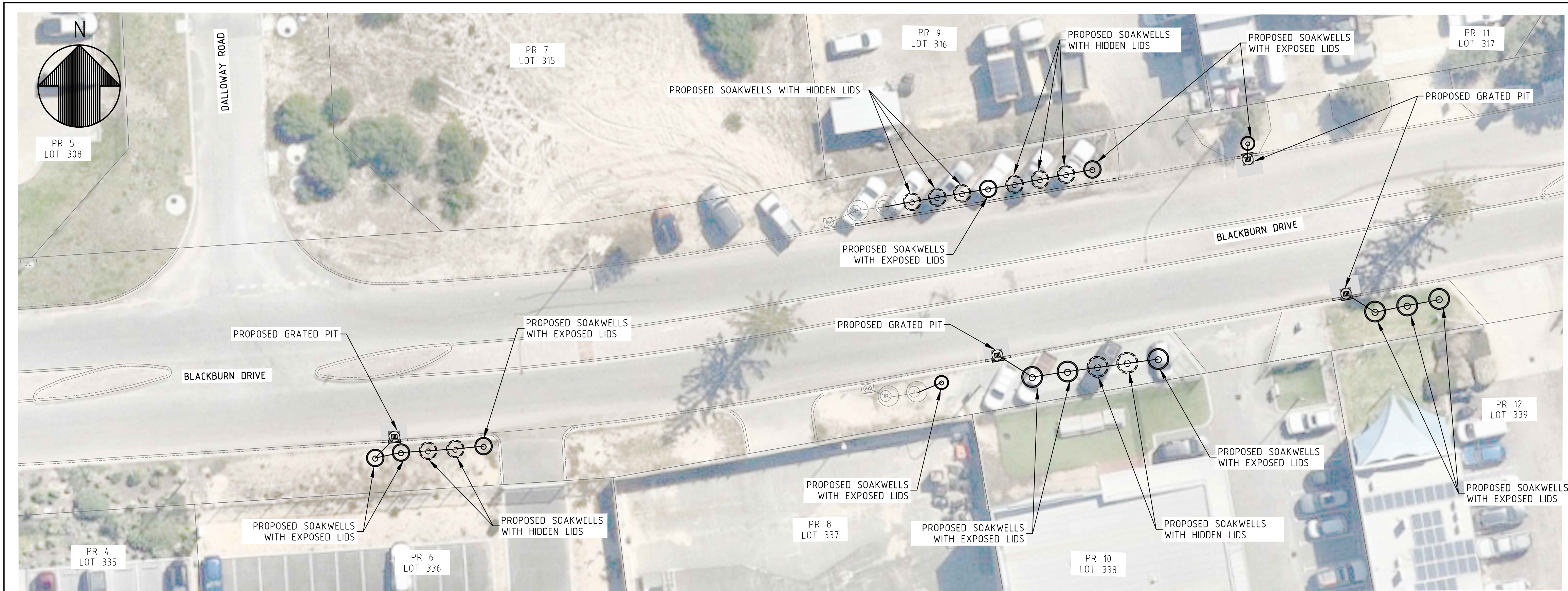
PLAN SCALE 1:250
