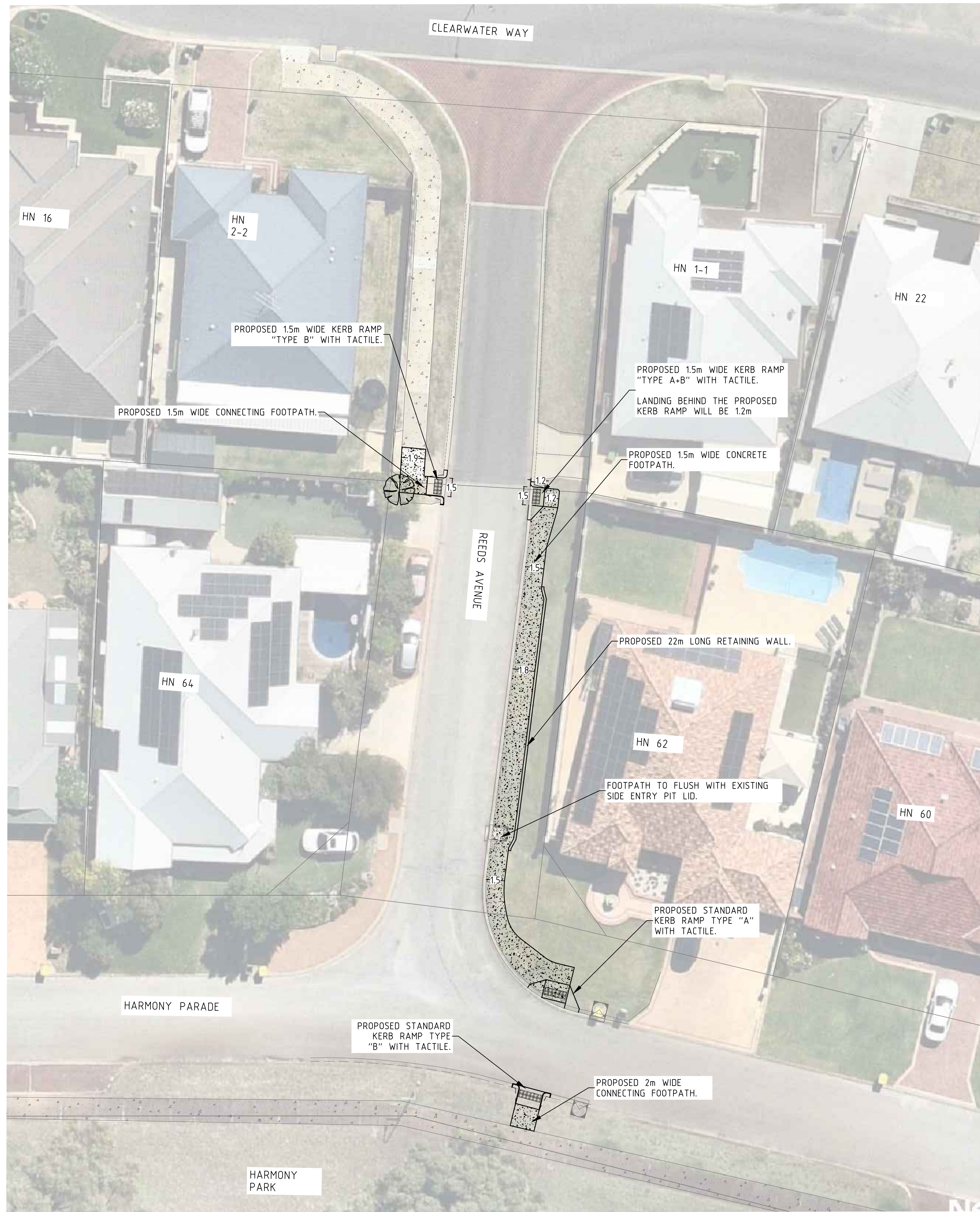
PLAN SCALE 1:200
