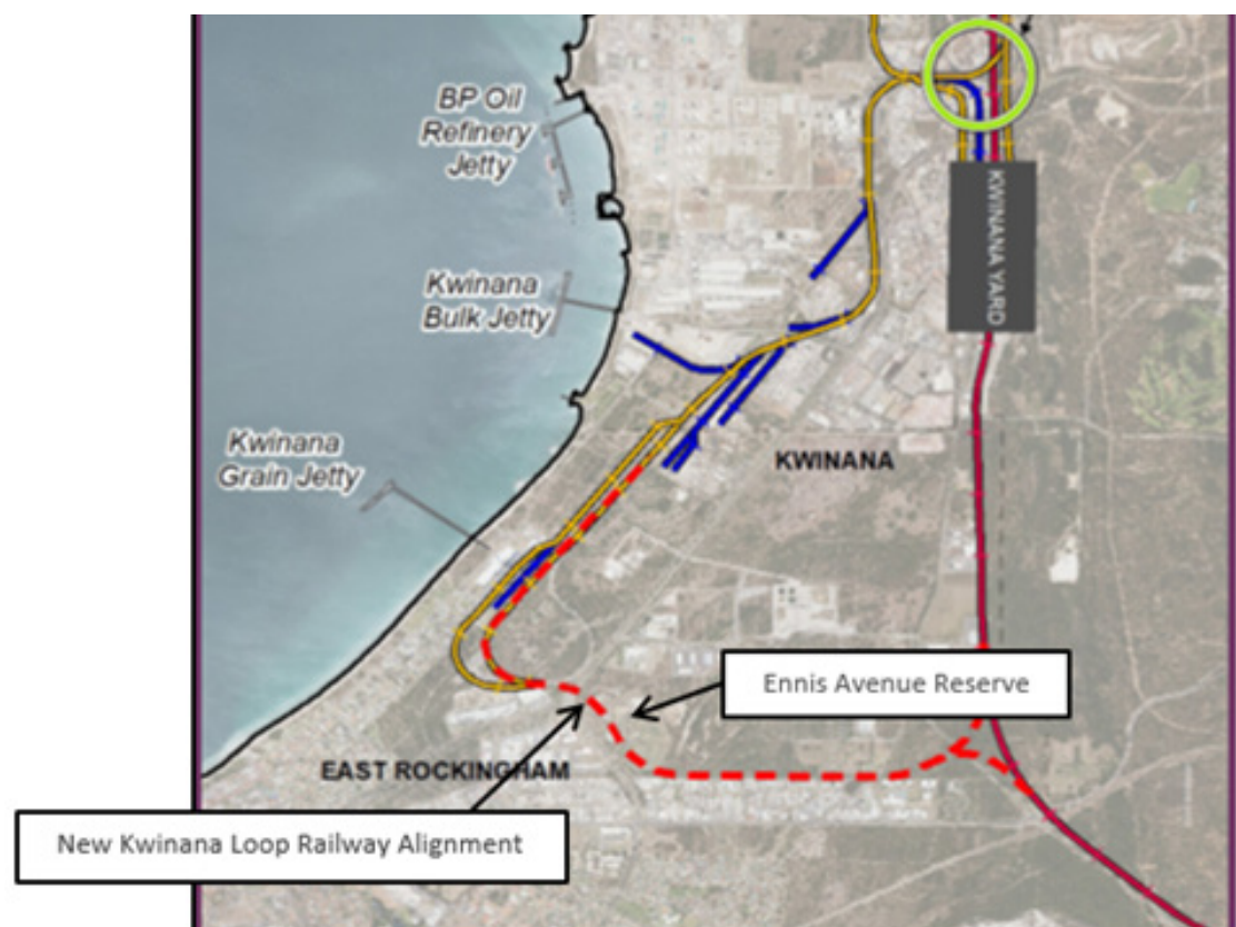
Figure 40: Proposed Kwinana Loop Railway Alignment
